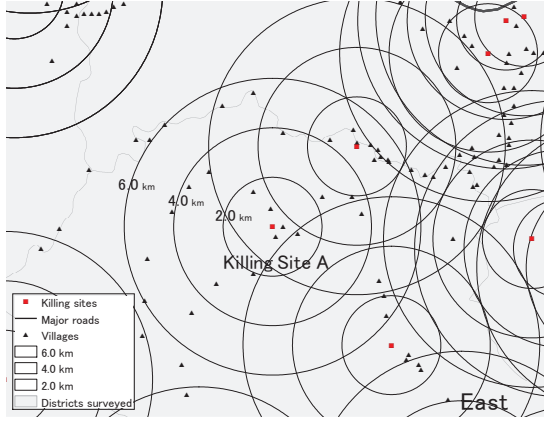
Figure 2: Spatial Clusters
